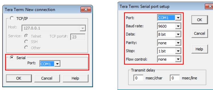
Figure 1-5: TeraTerm Pro Settings
