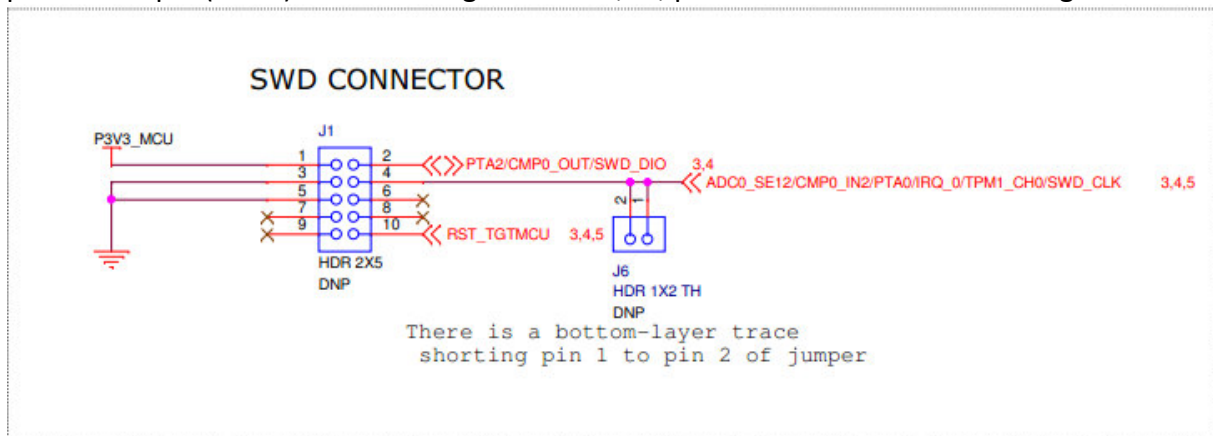
Figure 4. SWD connector
