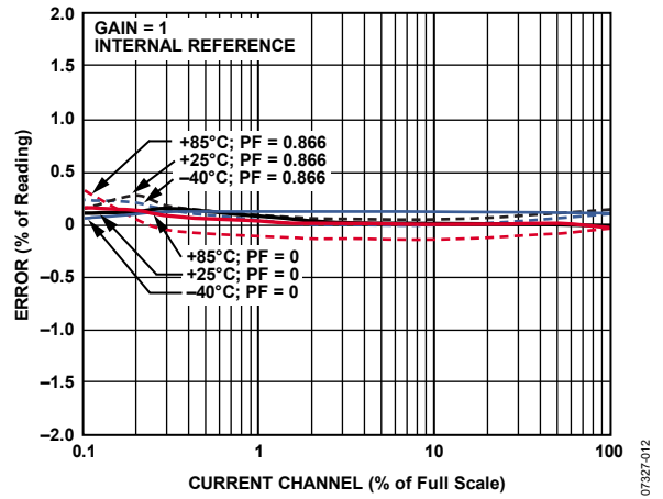
Figure 12. Reactive Energy Error as a Percentage of Reading (Gain = 1) over Power Factor with Internal Reference
