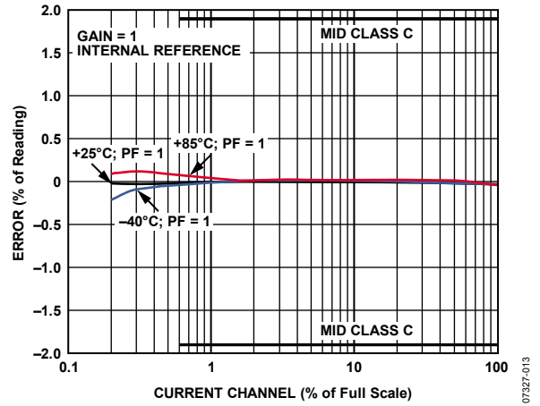
Figure 13. Current RMS Error as a Percentage of Reading (Gain = 1) over Temperature with Internal Reference
