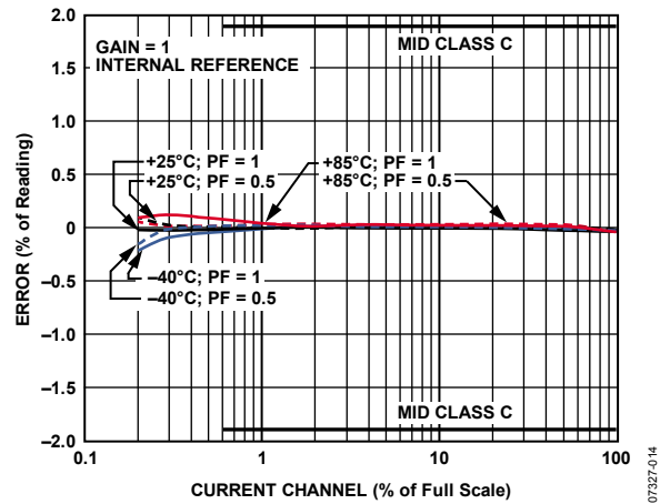
Figure 14. Current RMS Error as a Percentage of Reading (Gain = 1) over Power Factor with Internal Reference
