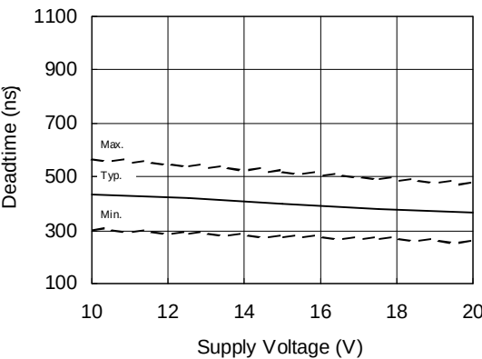
Figure 18B. Deadtime vs. Supply Voltage
