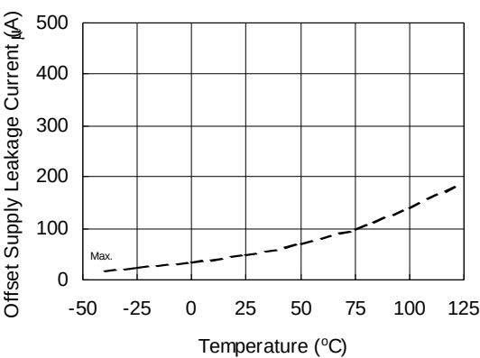
Figure 25A. Offset Supply Leakage Current vs. Temperature
