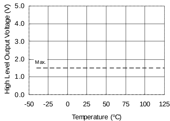
Figure 23A. High Level Output Voltage vs. Temperature ( I_O = 0\text{ mA} )
