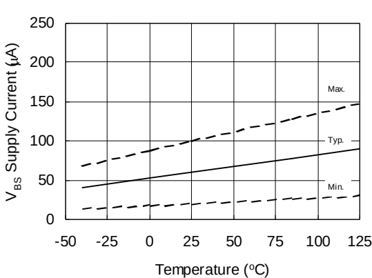
Figure 26A. V BS Supply Current vs. Temperature
