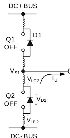
Figure 11: V_S negative
