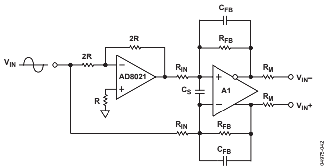
Figure 53. Single-Ended-to-Differential Conversion
