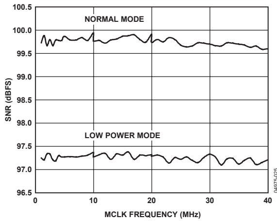
Figure 24. SNR vs. MCLK Frequency, 8x Decimation, -6 dB, 1 kHz Input Tone
