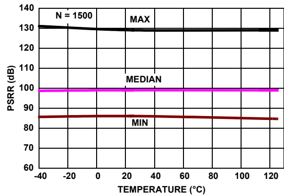
FIGURE 26. EL8172 PSRR vs TEMPERATURE, V_+, V_- = \pm 1.2V \text{ TO } \pm 2.5V
