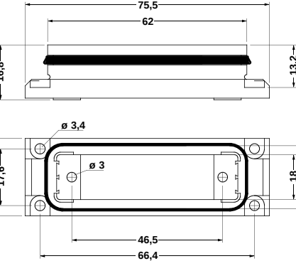
Dimensional drawing of panel mounting frame
