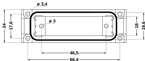
Dimensional drawing of panel mounting frame
