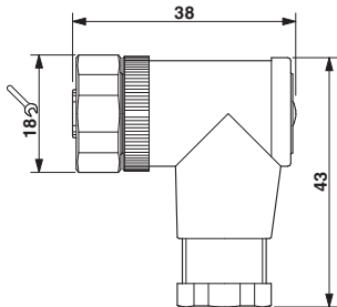
Dimensioned drawing
