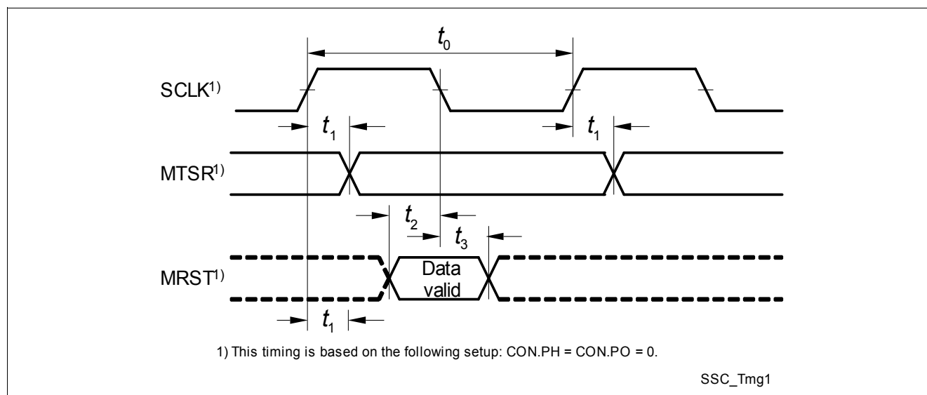
Figure 41 SSC Master Mode Timing
