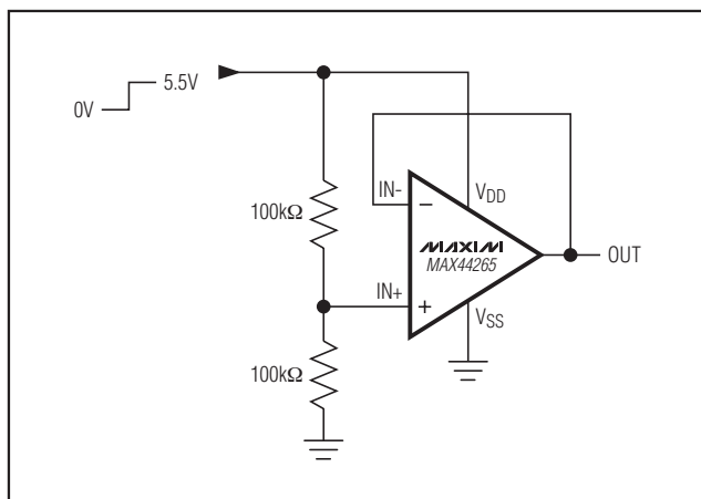
Figure 3. Power-Up Test Configuration
