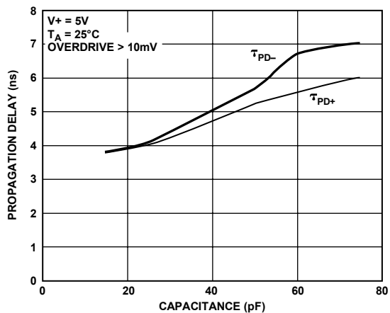
Figure 9. Propagation Delay vs. Load Capacitance
