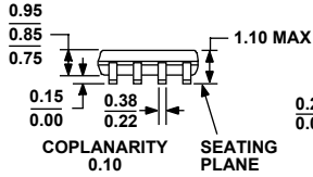
Figure 27. 8-Lead Mini Small Outline Package [MSOP] (RM-8)
