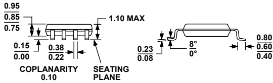
Figure 27. 8-Lead Mini Small Outline Package [MSOP] (RM-8)
