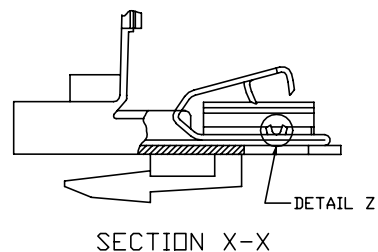
SECTION X-X
