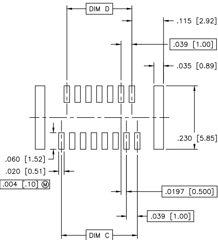
RECOMMENDED STENCIL LAYOUT FOR RECEPTACLE
