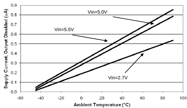
Supply Current, Output Disabled vs Ambient Temperature
