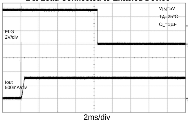
2 Ω Load Connected to Enabled Device
