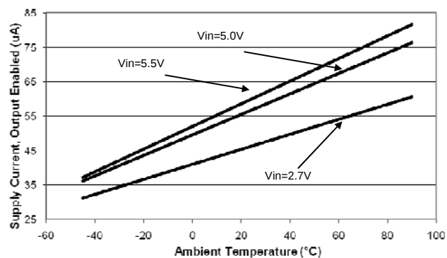
Supply Current, Output Enabled vs Ambient Temperature
