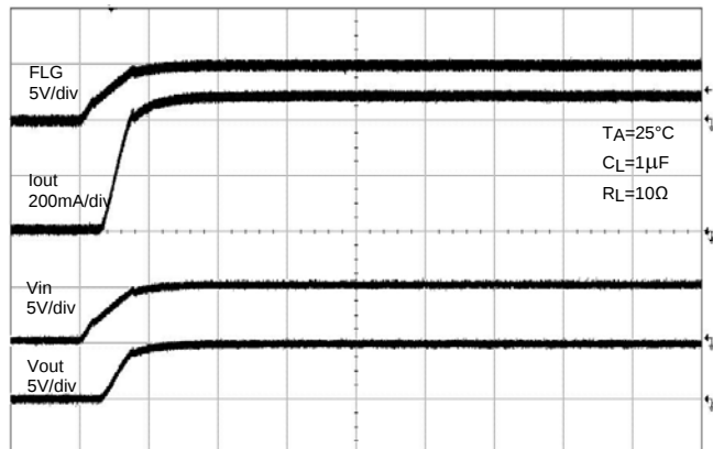
Power On
