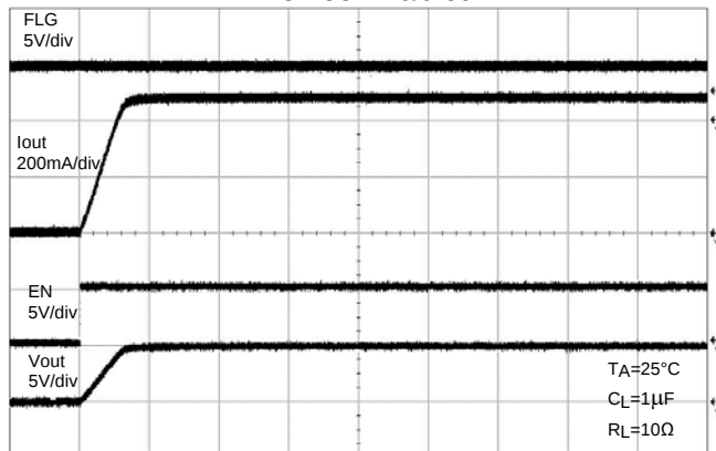
Device Enabled
