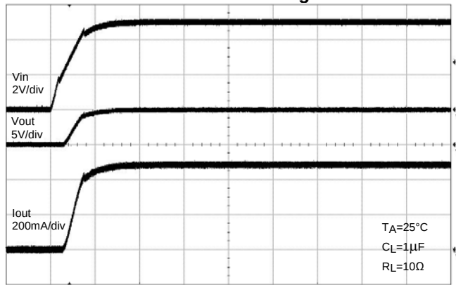
UVLO Increasing
