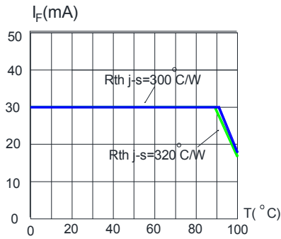
FIG. 3 RED&AMBER MAXIMUM FORWARD DC CURRENT VS SOLDER TEMPERATURE ( T_{jmax}=110\text{ }^\circ\text{C} )
