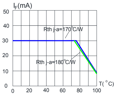
FIG. 5 RED&AMBER MAXIMUM FORWARD DC CURRENT VS AMBIENT TEMPERATURE ( T_{jmax}=110\text{ }^\circ\text{C} )
