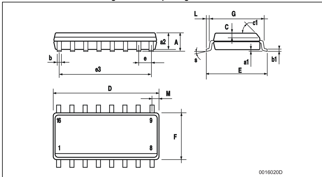
Figure 5. SO16 package outline
