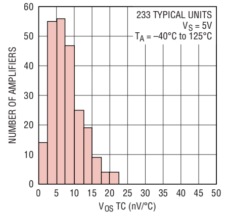
Input Offset Voltage Drift Distribution
