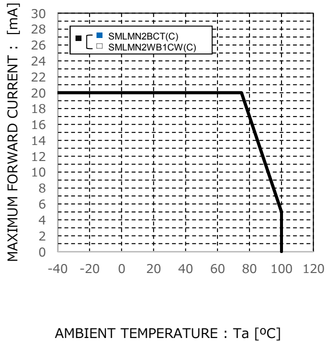
Fig.4 Derating
