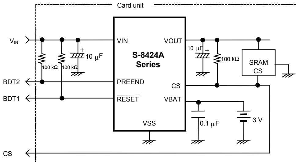
Figure 25 Application Circuit 3
