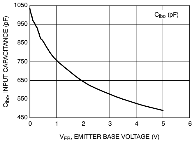
Figure 7. Input Capacitance
