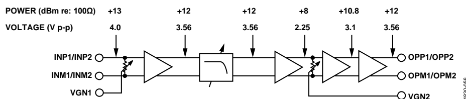
Figure 73. Maximum Signal Levels—Single Channel Shown
