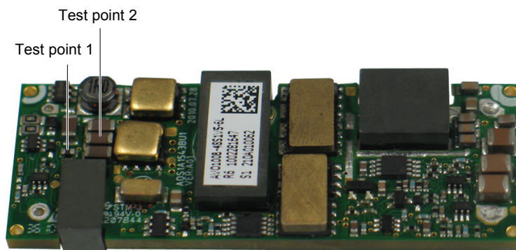
Figure 16 Thermal test point (top)
