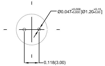
All dimensions in inches (mm)
