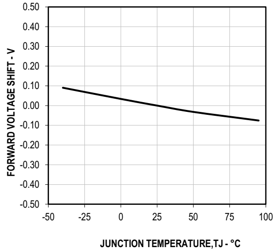
Figure 9: Forward Voltage vs. Temperature
