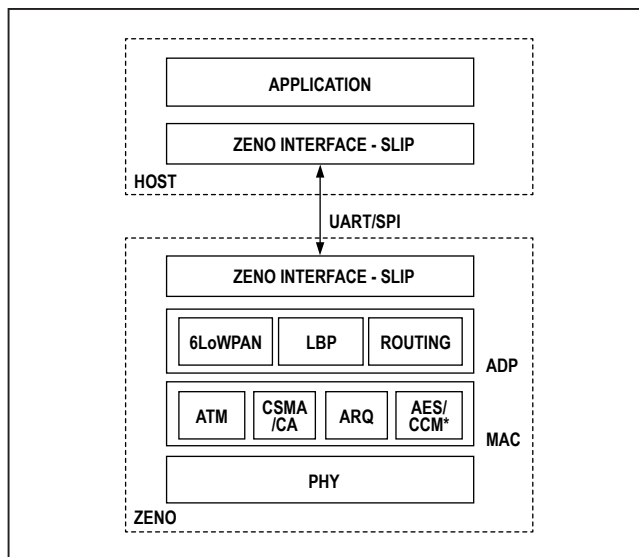
Figure 2 ZENO Architecture.
