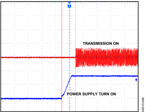
Figure 17. Time to Initialize, Including Reset, 40\text{ ms/DIV}
