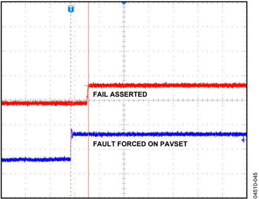
Figure 16. FAIL Assert Time, 1\text{ }\mu\text{s/DIV}
