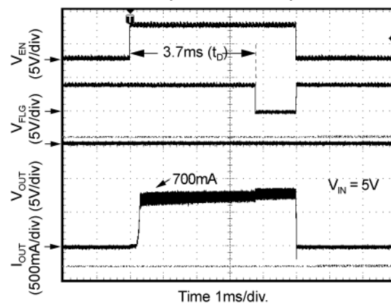
Enabled into Short (MIC2026A-1)
