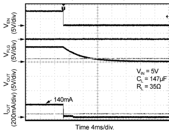
Turn-Off Zoom (MIC2026A-1)
