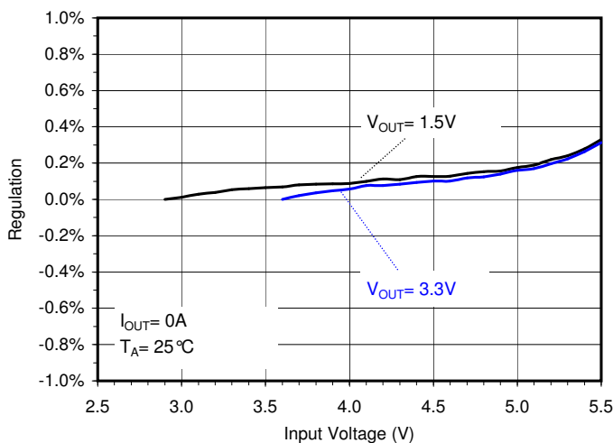
Line Regulation
