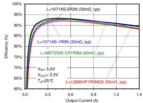
Figure 6 — Typical efficiency curves (V IN =5.0V, V OUT =3.3V)
