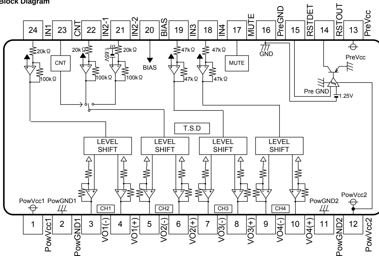
Fig.3:Block Diagram
