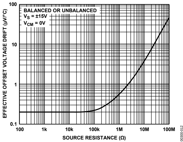
Figure 12. Effective TCV_{OS} vs. Source Resistance
