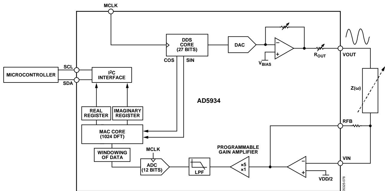
Figure 14. Block Overview
