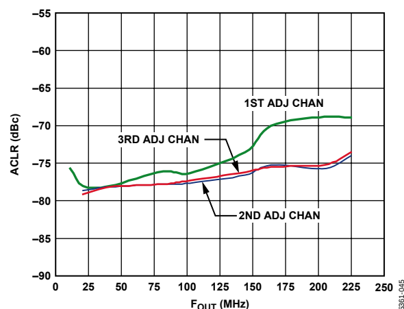
Figure 48. AD9776 ACLR, f_{\text{DATA}} = 122.88\text{ MSPS} , 4× Interpolation, f_{\text{DAC}}/4 Modulation
