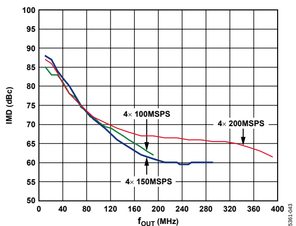
Figure 46. AD9776 IMD, 4× Interpolation
