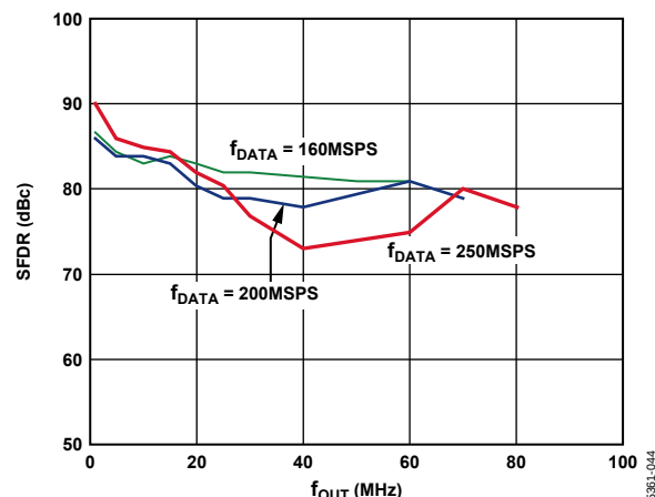
Figure 47. AD9776 In-Band SFDR, 2× Interpolation
