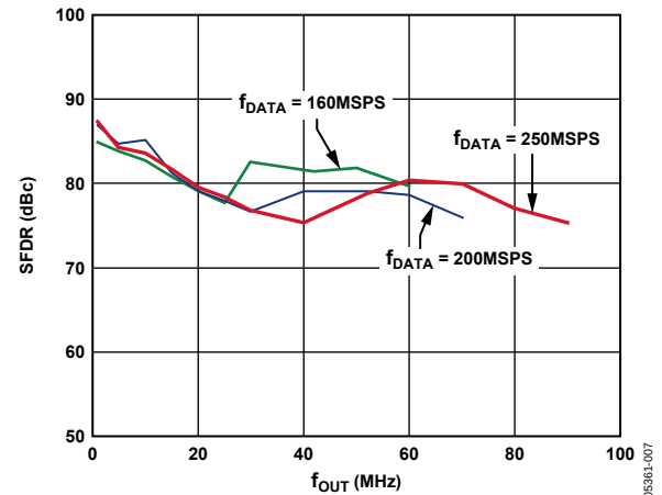
Figure 8. AD9779 In-Band SFDR vs. f_{OUT} , 1 \times Interpolation
