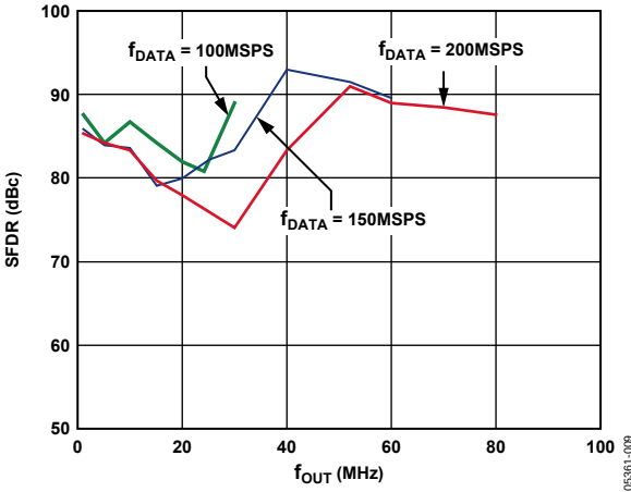
Figure 10. AD9779 In-Band SFDR vs. f_{OUT} , 4 \times Interpolation
