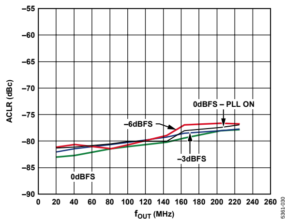
Figure 33. AD9779 ACLR for Third Adjacent Band WCDMA, 4x Interpolation, f_{DATA} = 122.88 MSPS, On-Chip Modulation Translates Baseband Signal to IF
