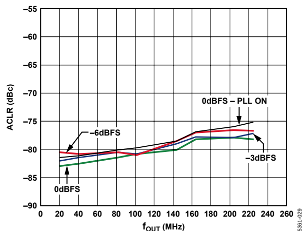
Figure 32. AD9779 ACLR for Second Adjacent Band WCDMA, 4x Interpolation, f_{DATA} = 122.88 MSPS, On-Chip Modulation Translates Baseband Signal to IF
