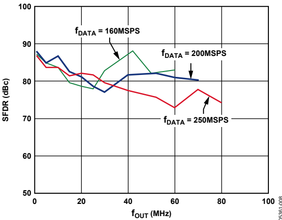
Figure 9. AD9779 In-Band SFDR vs. f_{OUT} , 2 \times Interpolation
