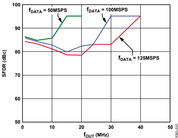
Figure 11. AD9779 In-Band SFDR vs. f_{OUT} , 8 \times Interpolation
