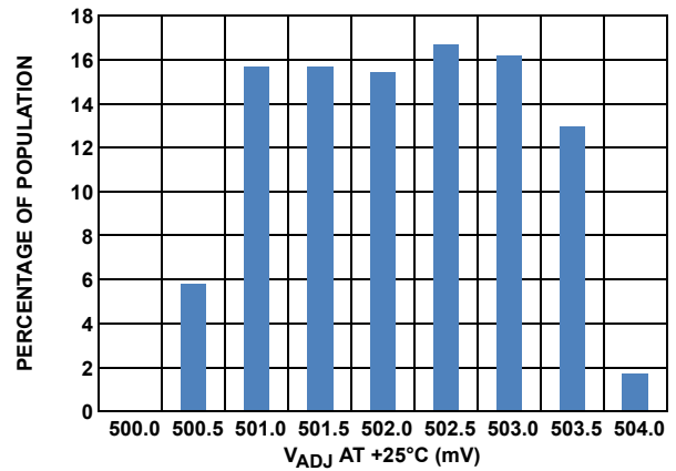
FIGURE 7. V ADJ DISTRIBUTION
