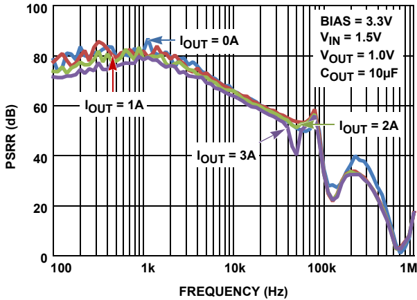
FIGURE 30. V_{IN} PSRR vs FREQUENCY FOR VARIOUS LOAD CURRENTS
