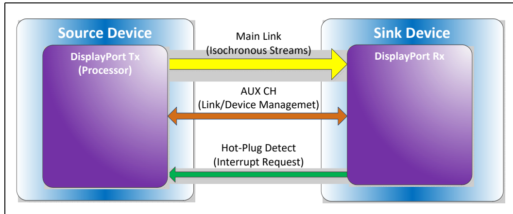
Figure 2-8. DisplayPort Overview
