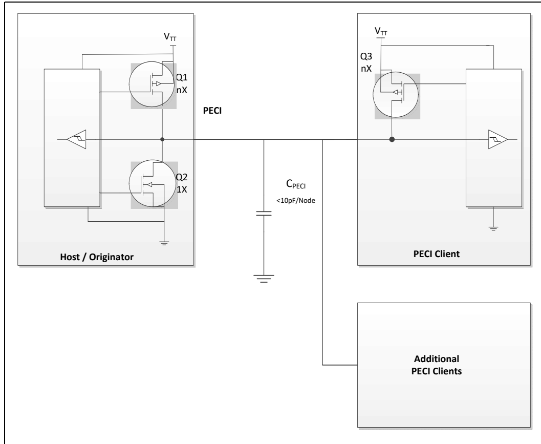
Figure 2-10. Example for PECE Host-Clients Connection
