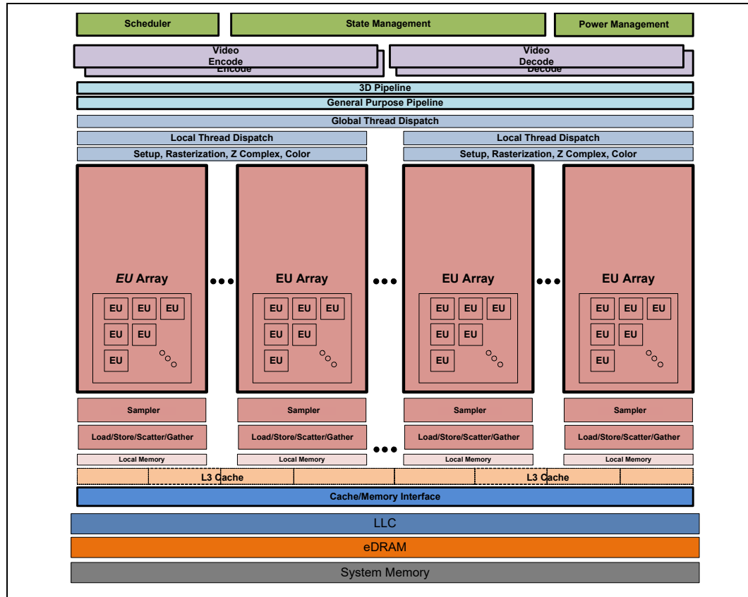
Figure 2-6. Gen 9 LP Block Diagram
