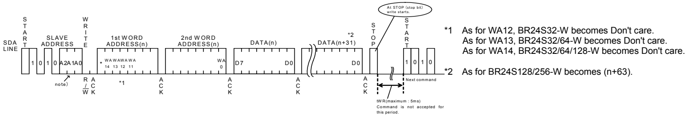
Fig.39 Page write cycle(BR24S32/64/128/256-W)
