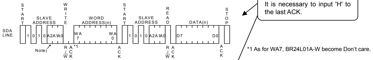
Fig.43 Random read cycle (BR24L01A/02/04/08/16-W)
