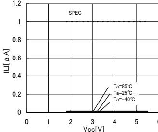
Fig.7 Input leak current ILI (SCL,WP)
