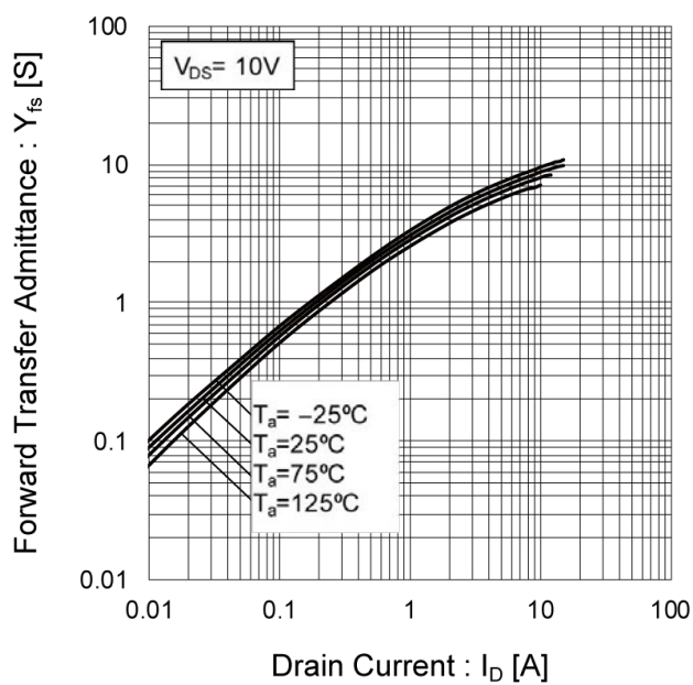
Fig.12 Forward Transfer Admittance vs. Drain Current
