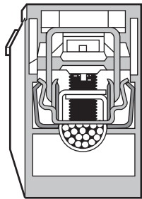
Figure 3. Unique Cable Termination
