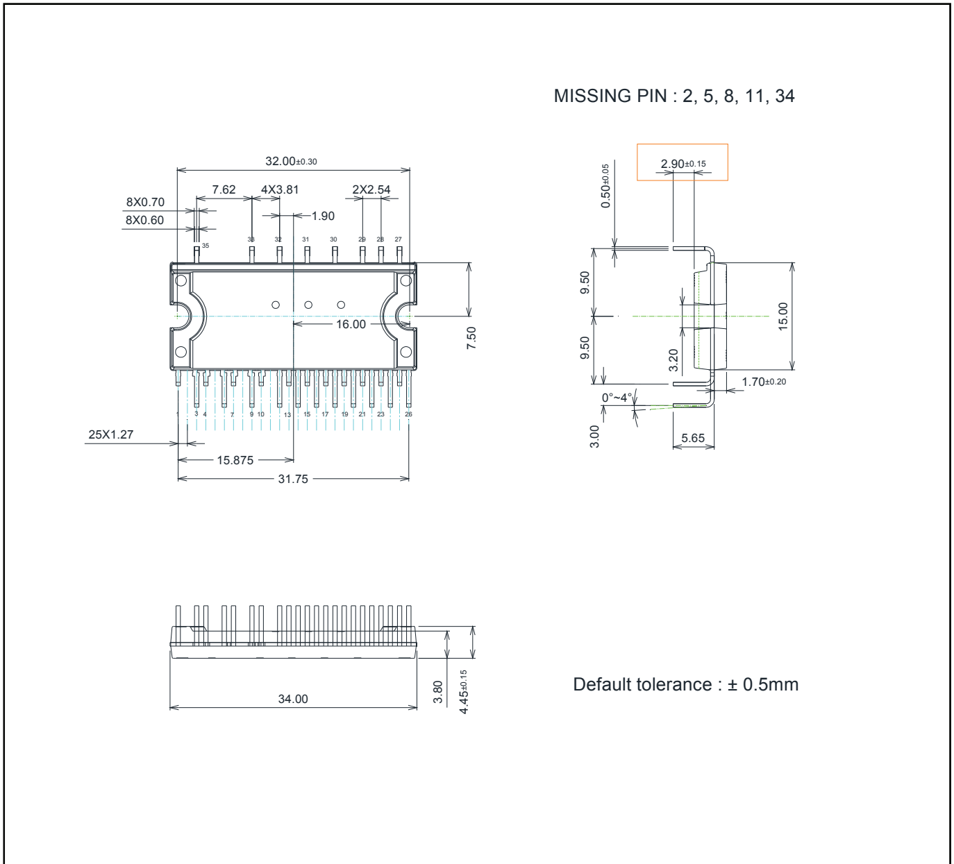
Figure 19 IM393-S6E2
