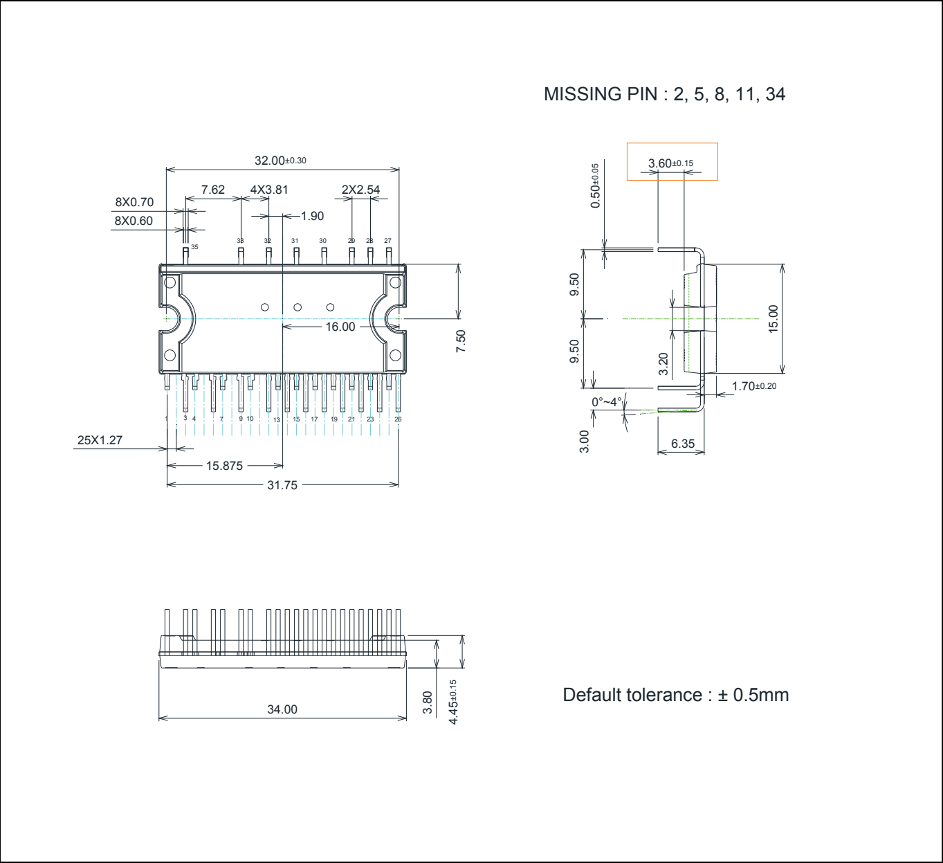
Figure 20 IM393-S6E3
