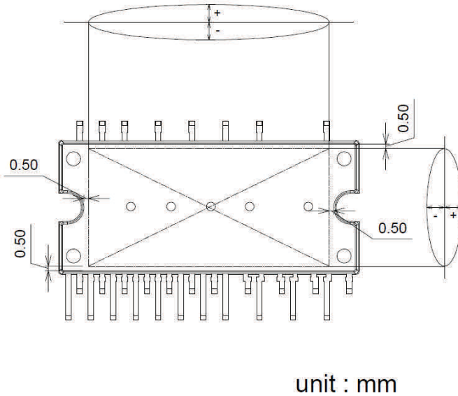
Figure 8 Backside curvature measurement position
