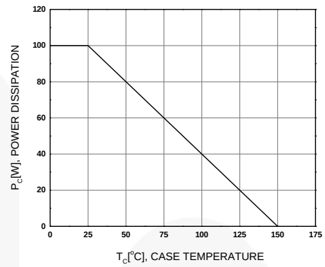
Figure 8. Power Derating
