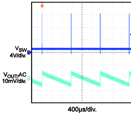
Steady State I_{OUT} = 0\text{ A} , Pulse Skip
