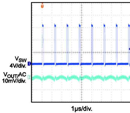
Steady State I_{OUT} = 0\text{ A} , Forced CCM
