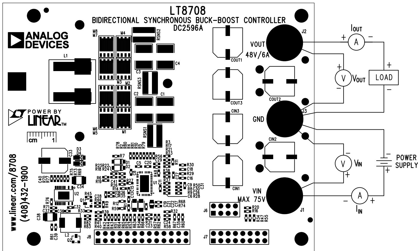
Figure 2. Test Setup
